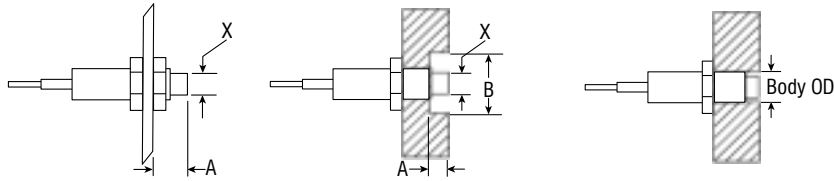
Bracket Mount
