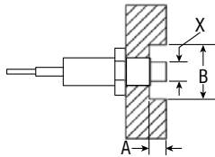
Flush Mount With Counterbore
